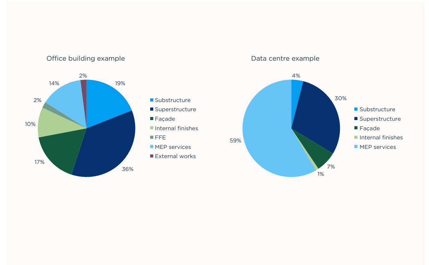
Figure 5 Whole life embodied carbon element comparison ▼
